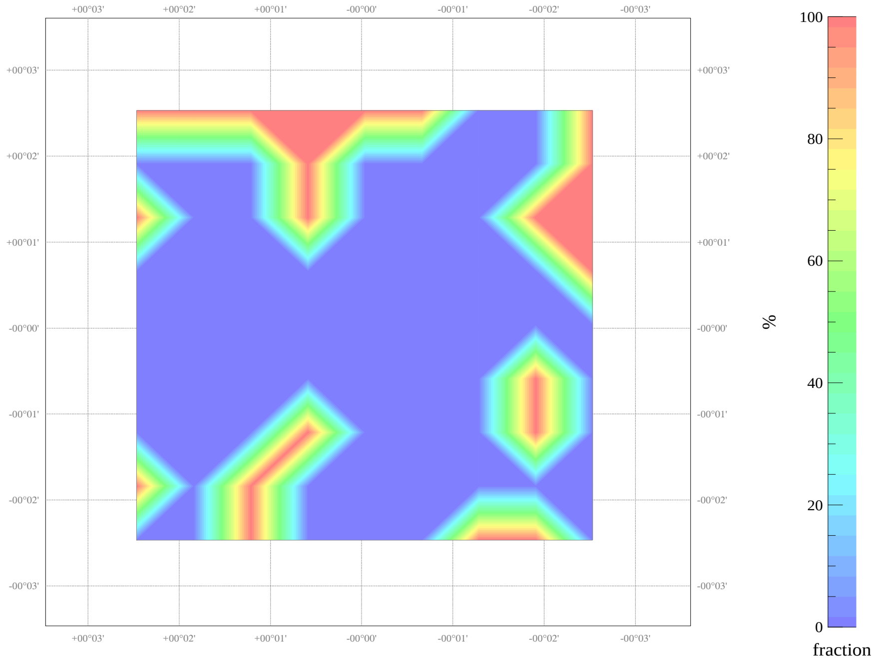
Field NGC_5846: source count fraction map
