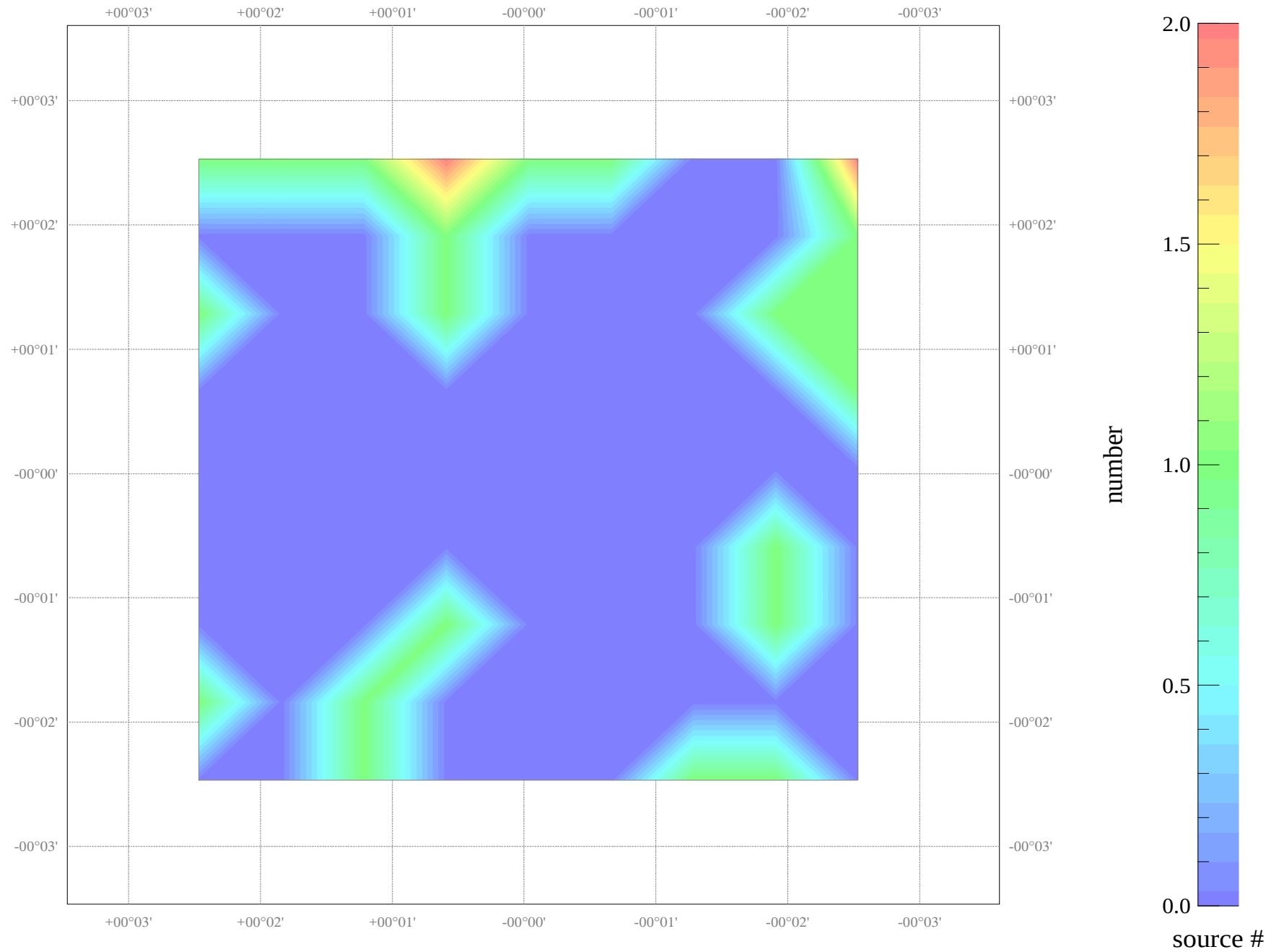
Field NGC_5846: source count map
