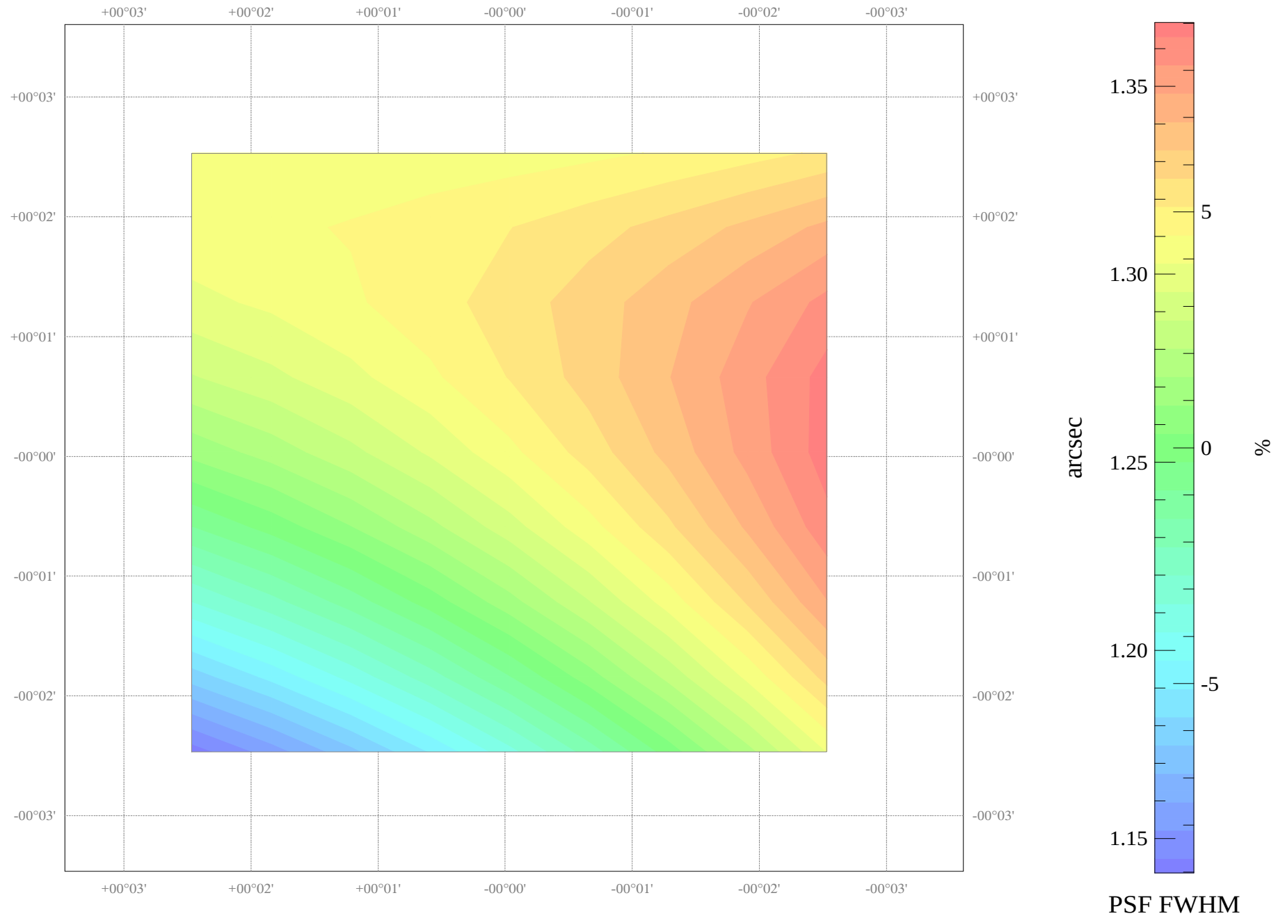
Field NGC_5846: FWHM map
