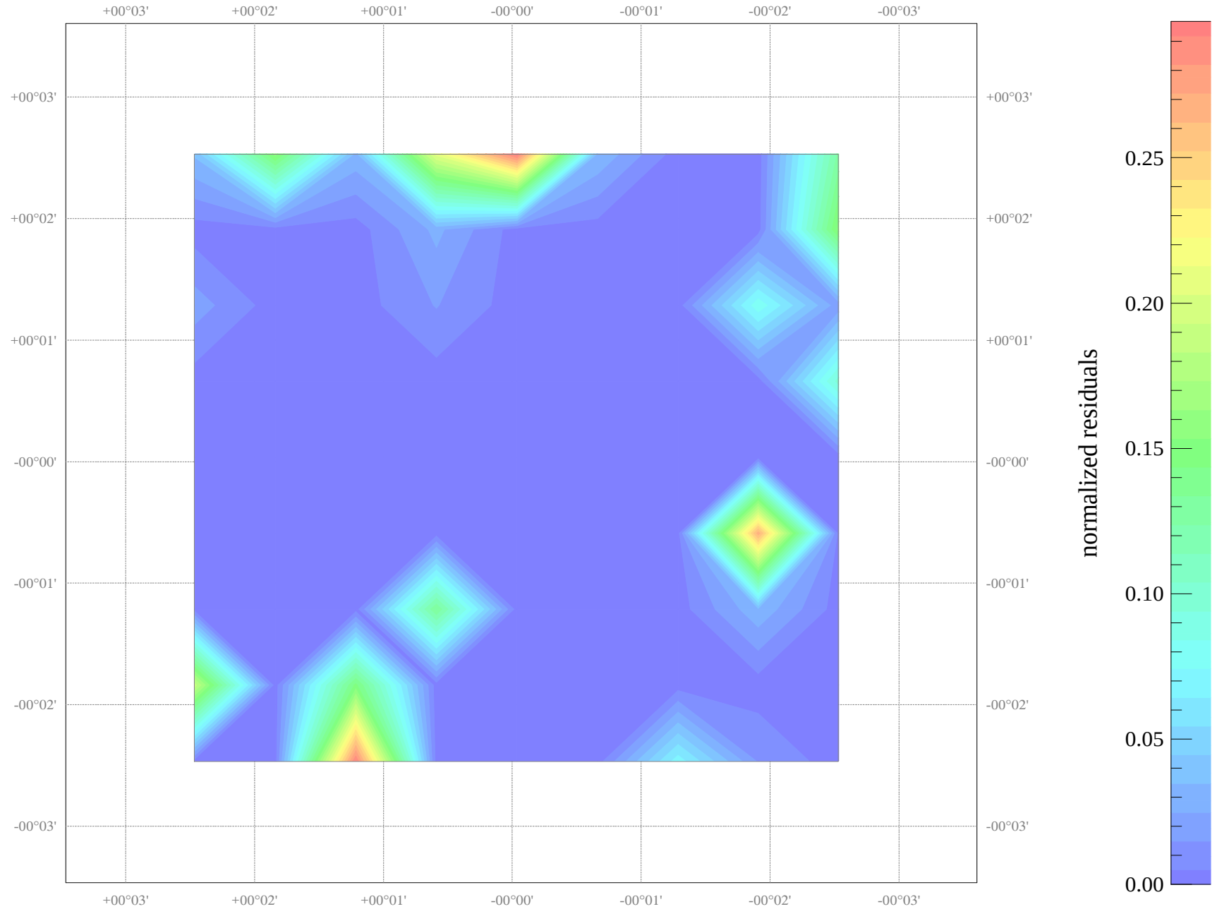
Field NGC_5846: map of residuals
