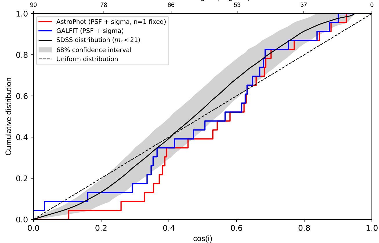
CDF Bias Comparison: AstroPhot n=1 fixed vs GALFIT (PSF + sigma)
