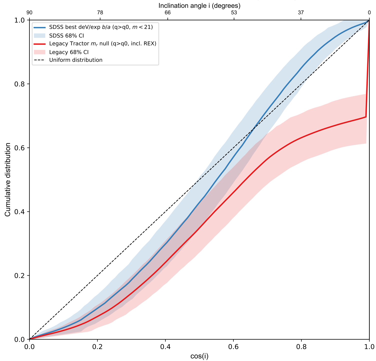
Null CDF: SDSS vs Legacy model m_r (strict, joint footprint)
