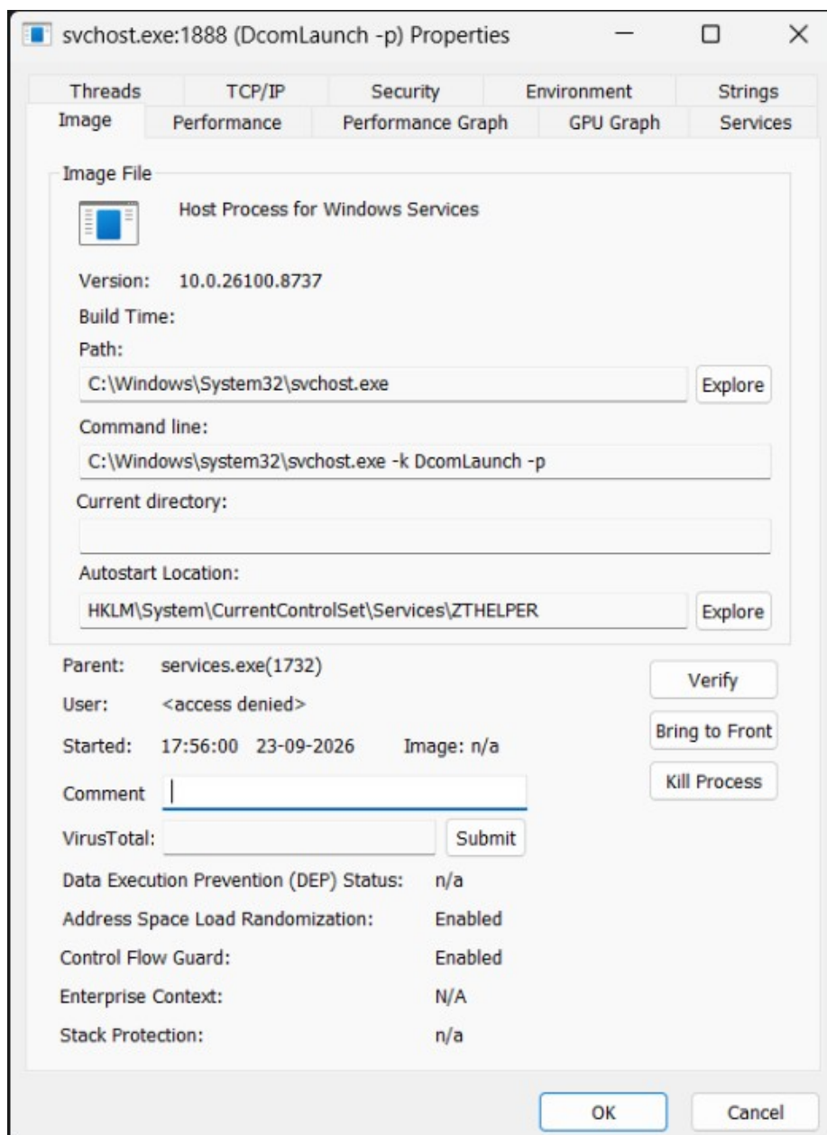
Screenshot 2 - Process properties
