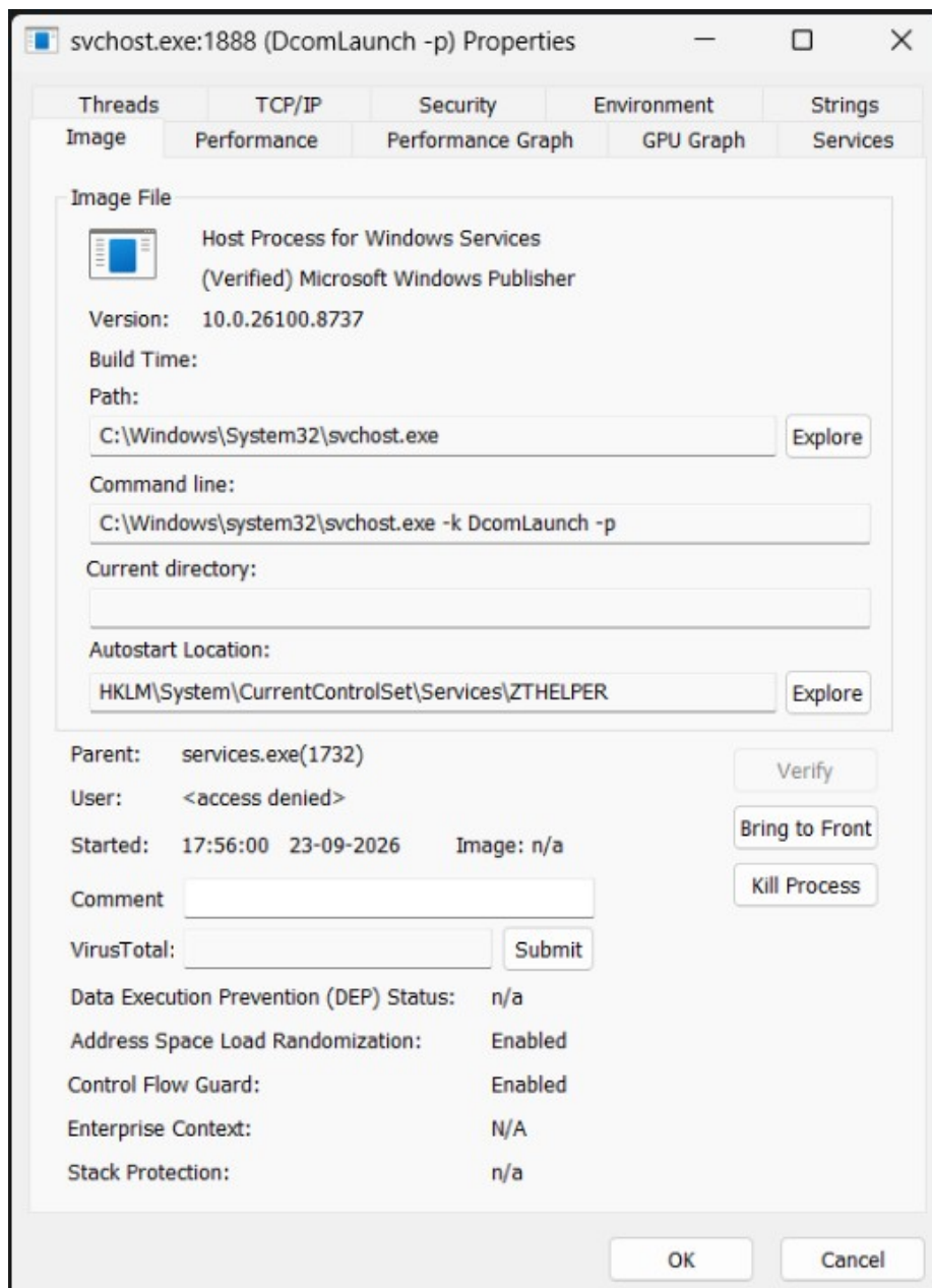
Screenshot 4 - Verified Microsoft Windows Publisher signature
