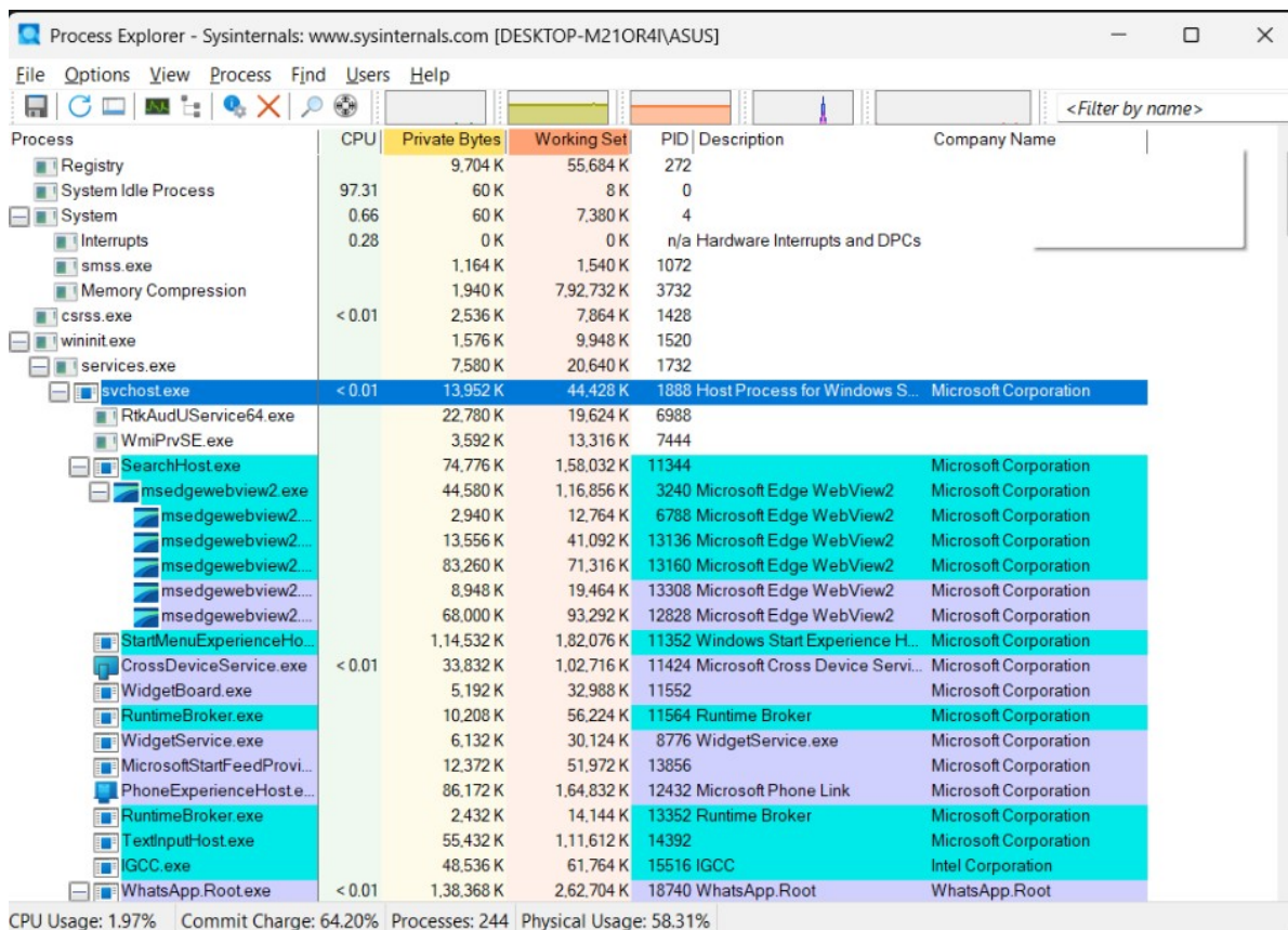
Screenshot 6 - Process analysis in Process Explorer
