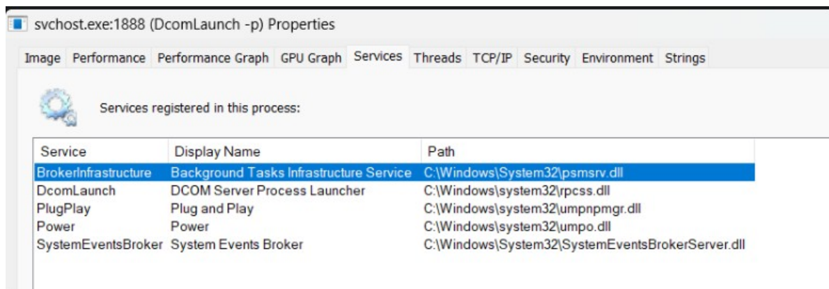
Screenshot 5 - Registered services
