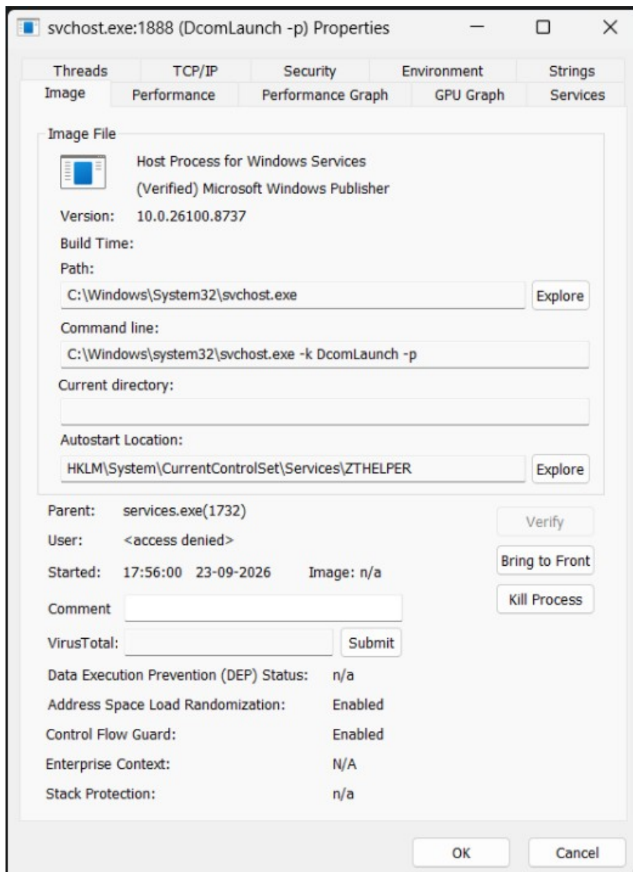
Screenshot 3 - svchost.exe process properties
