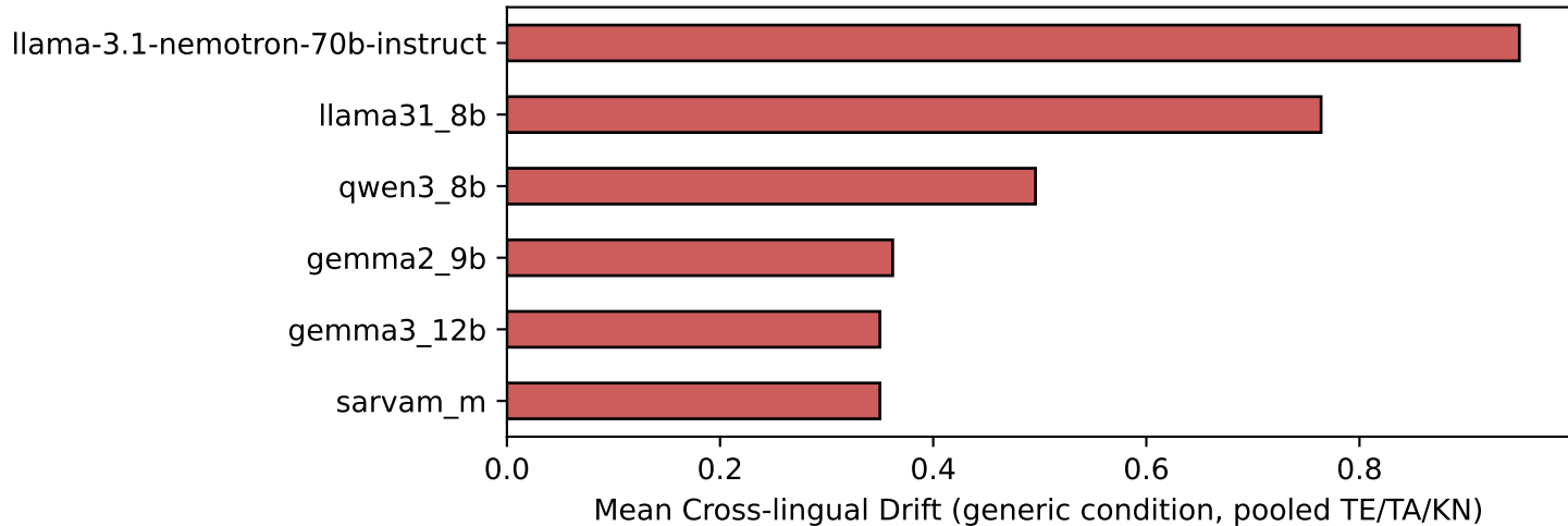
Model Ranking by Overall Cross-lingual Value Drift
