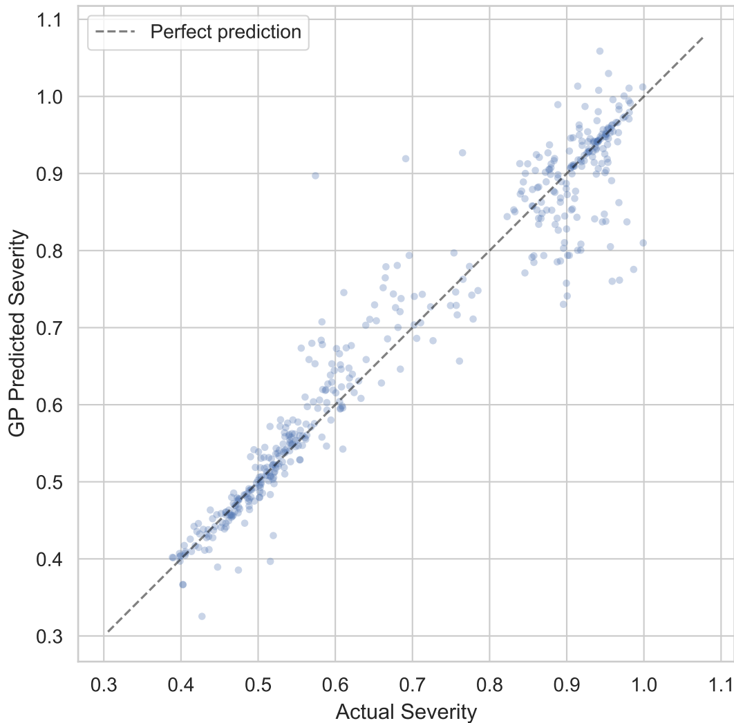
GP Surrogate: Joint 9D ( R^2=0.935 )
