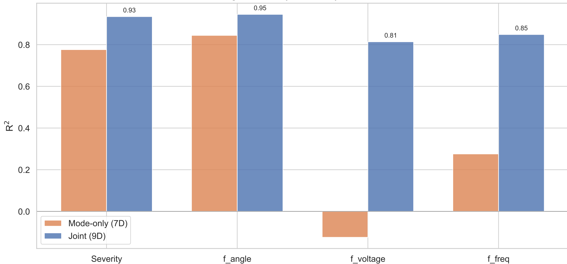
GP Surrogate Accuracy: Mode-only vs Joint Features
