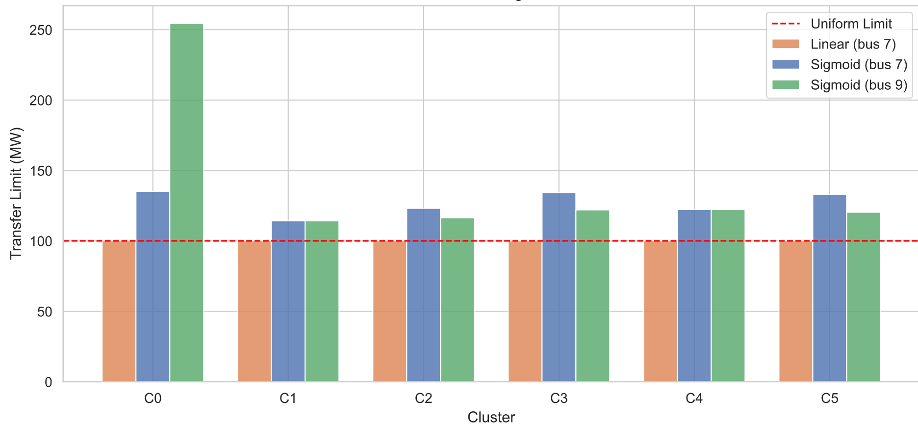
Tiered Limits: Linear vs Sigmoid vs Per-Fault
