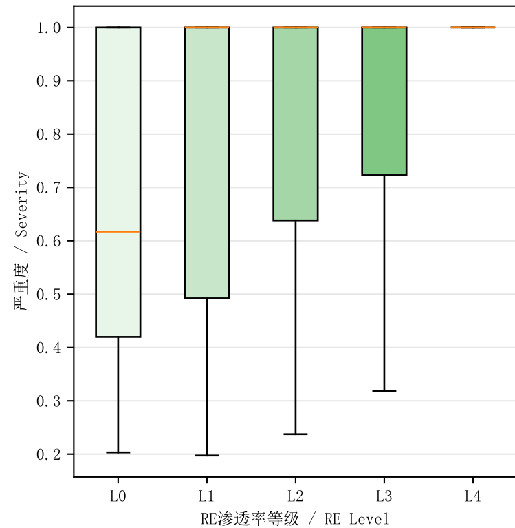
功角严重度 (Angle severity)
