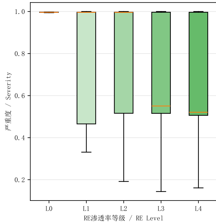
电压严重度 (Voltage severity)
