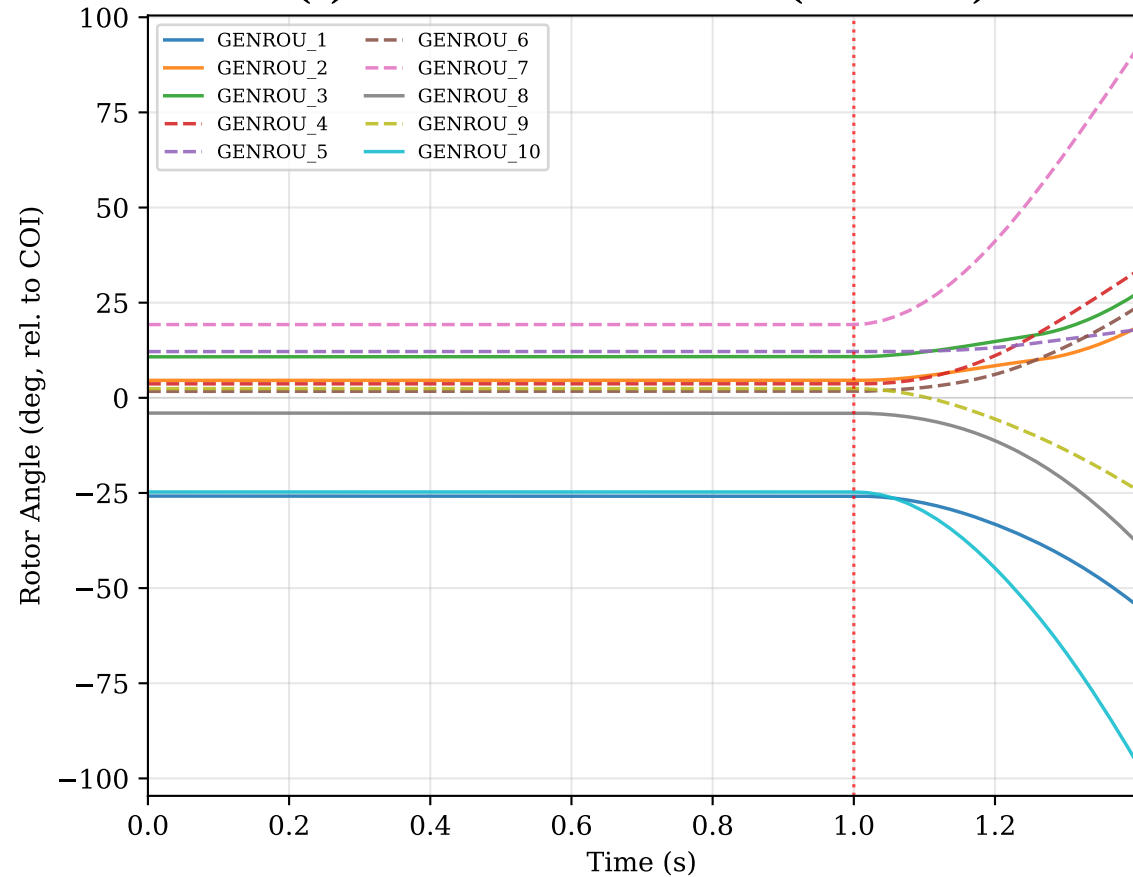
(a) Unstable: Bus16 ct=0.25s (sev=0.978)
