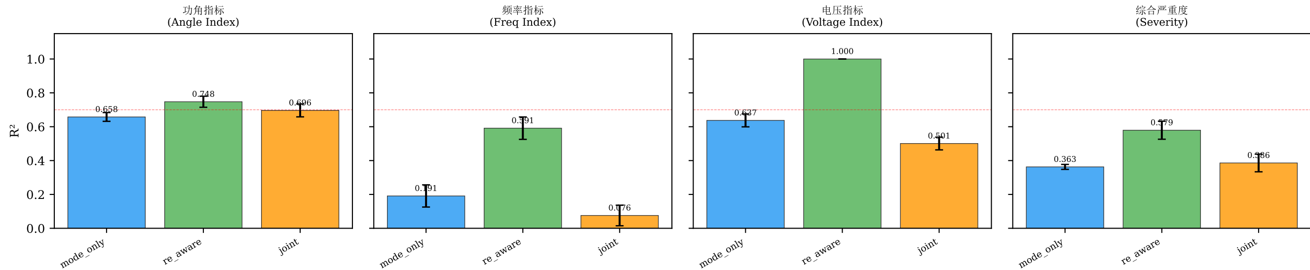
图3 多输出高斯过程代理模型精度对比 Fig. 3 Multi-output GP surrogate accuracy comparison
