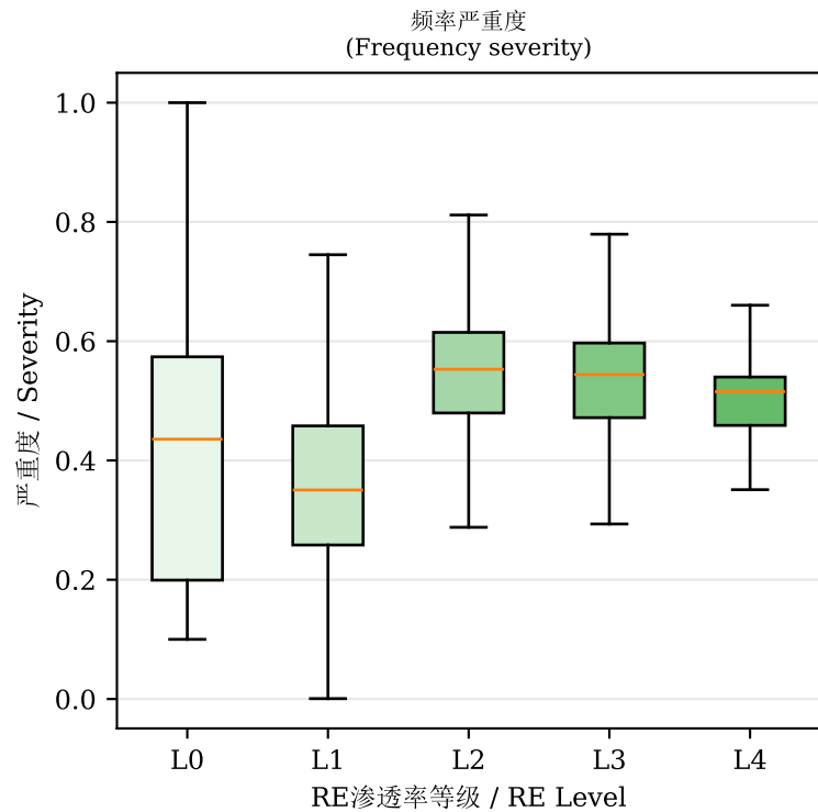
图5 新能源渗透率对约束严重度的影响 Fig. 5 Impact of RE penetration on constraint severity
