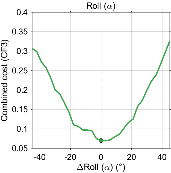
UAV: Angle sensitivity of camera 1 (GA-best, Uniform, sp=1.00 m, 7 cams)
