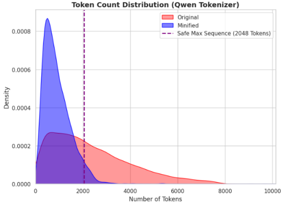
Figure 4: Structural representation of the training SVGs in tokens before and after minimization and preprocessing pipeline.
