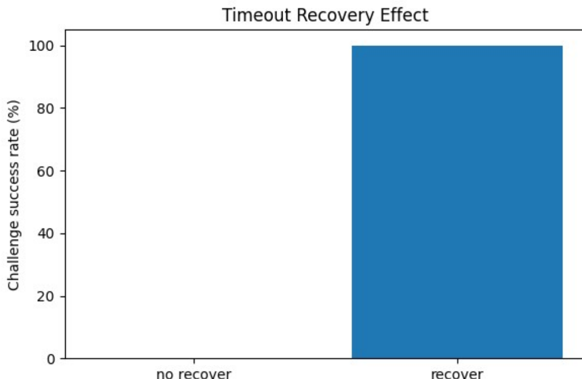
图 6 timeout recover 对挑战完成率的影响 Fig.6 Effect of Timeout Recovery on Challenge Completion
