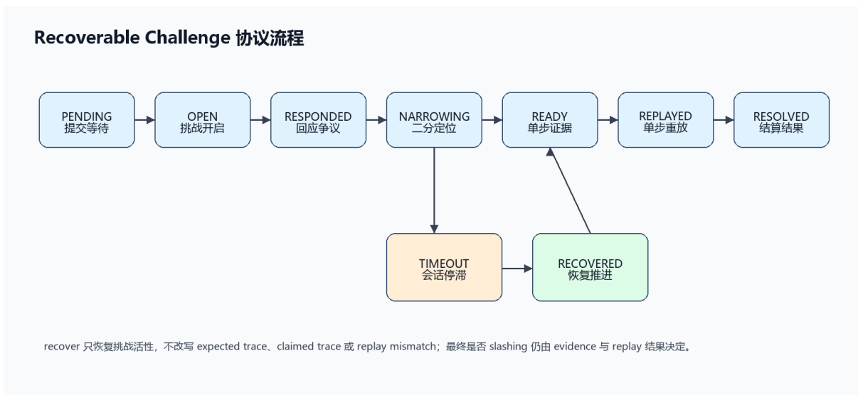
图 2 Recoverable Challenge 协议流程 Fig.2 Workflow of the Recoverable Challenge Protocol
