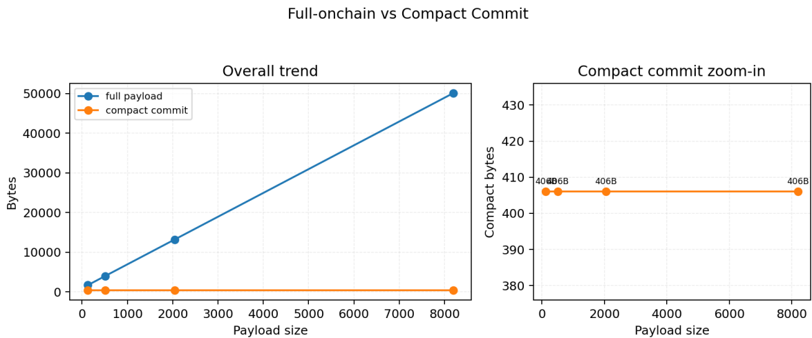
图3 full payload 与 compact commit 的字节规模对比 Fig.3 Byte Size Comparison between Full Payload and Compact Commit
