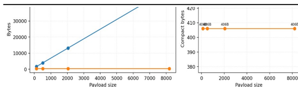
图 3 完整负载与紧凑提交的字节规模对比 Fig.3 Byte-size comparison between full payloads and compact commits
