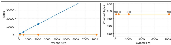
图 3 完整负载与紧凑提交的字节规模对比 Fig.3 Byte-size comparison between full payloads and compact commits
