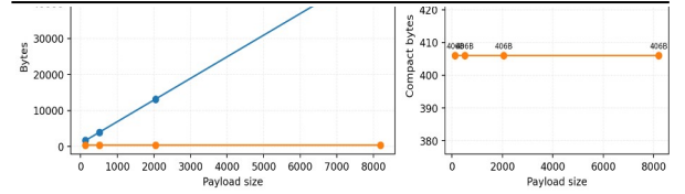
图 3 完整负载与紧凑提交的字节规模对比 Fig.3 Byte-size comparison between full payloads and compact commits
