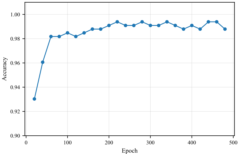
Epoch vs Accuracy
