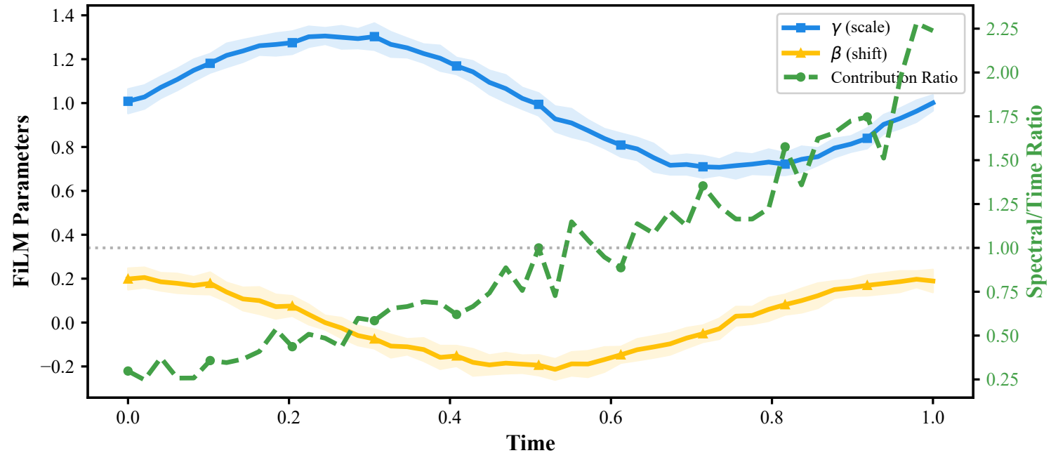
FiLM Temporal Adaptation
