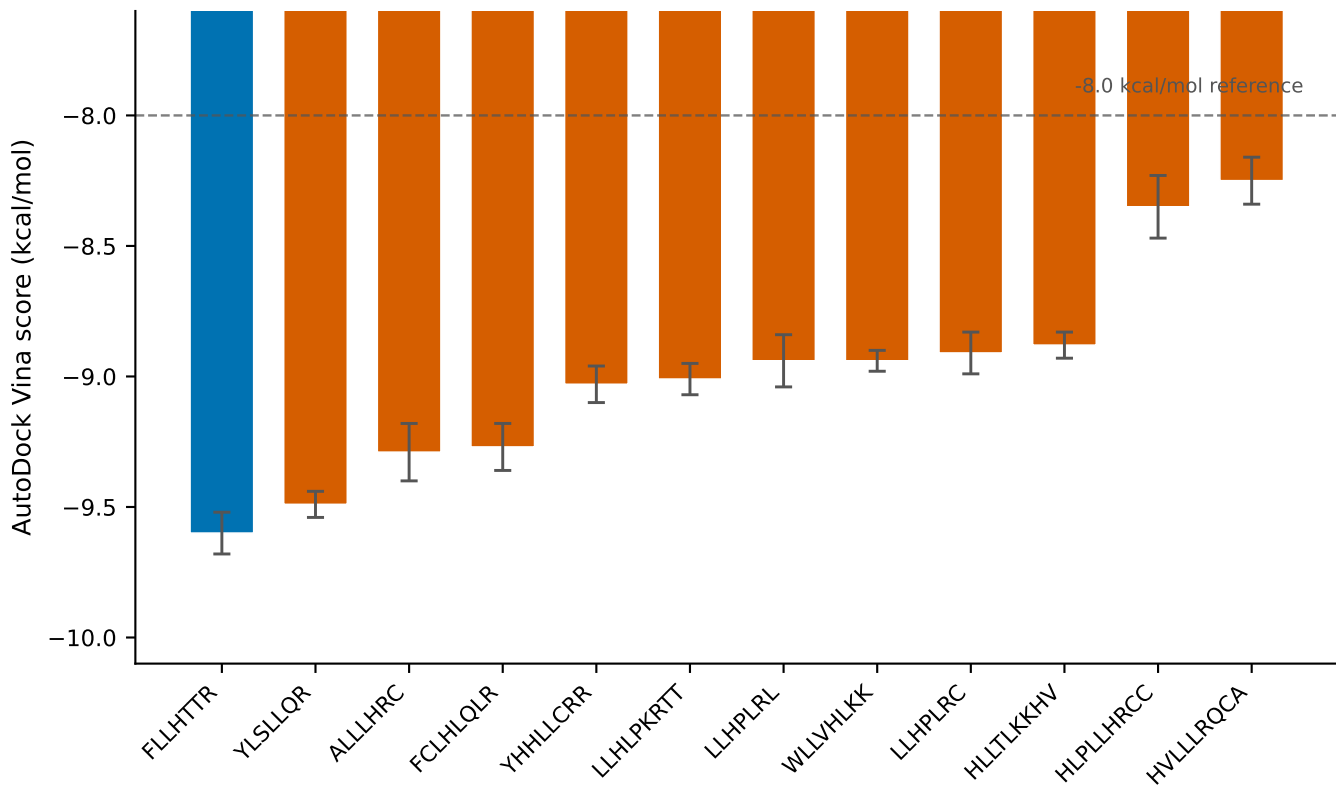
PAS-focused docking against human AChE (PDB 4EY6)
