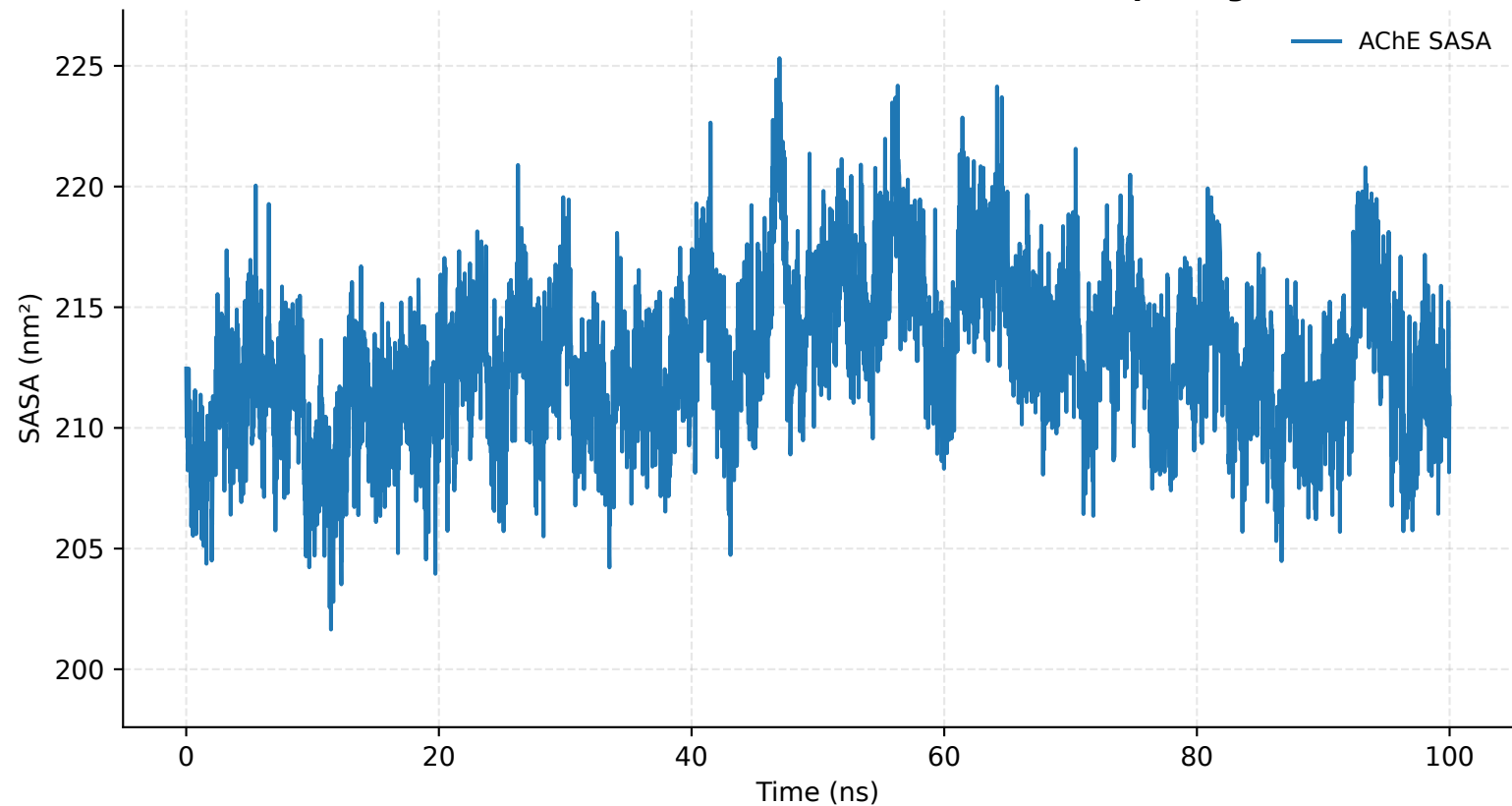
Solvent Accessible Surface Area (AChE SASA, Paper Fig 3)
