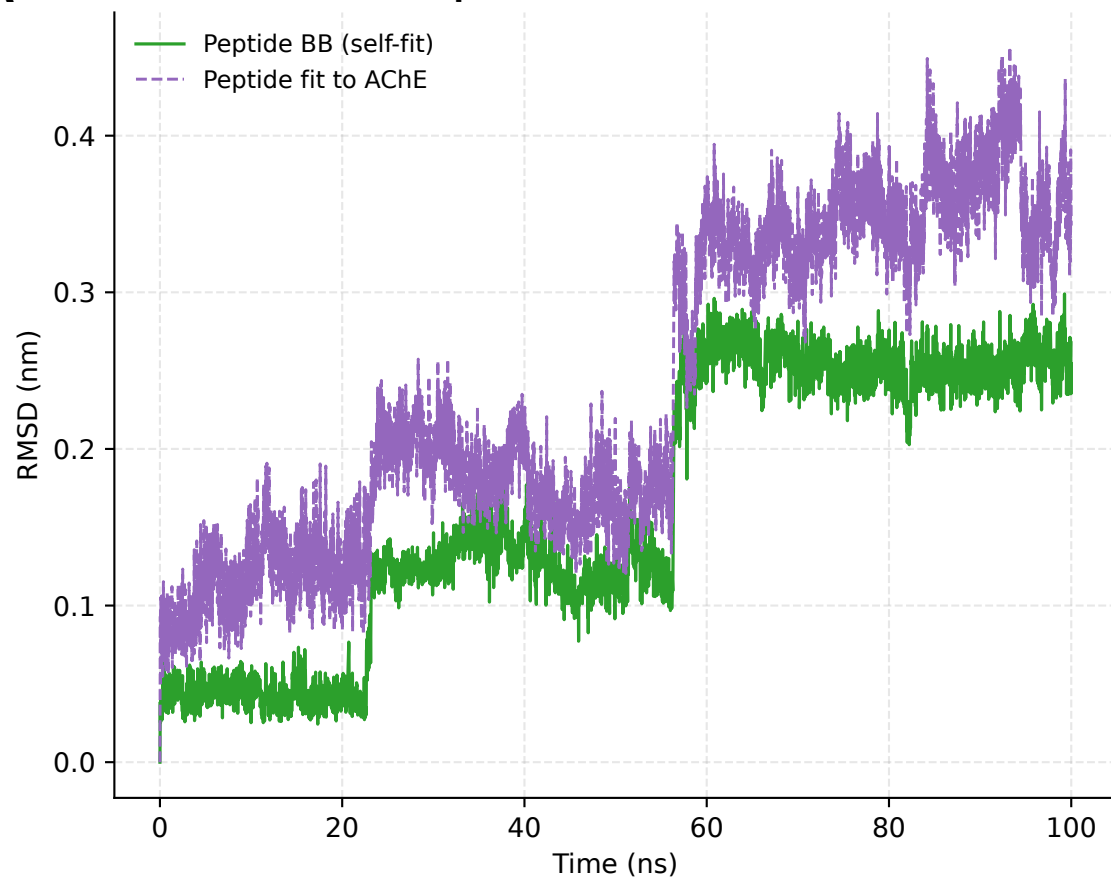
Peptide Backbone RMSD
