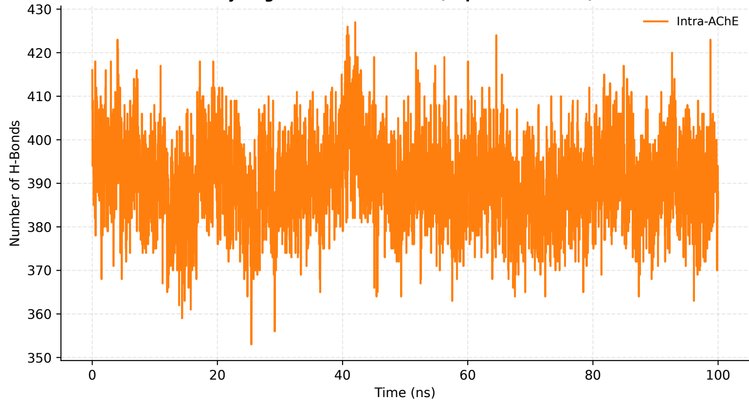
Hydrogen Bonds over Time (Paper Section 3.3)
