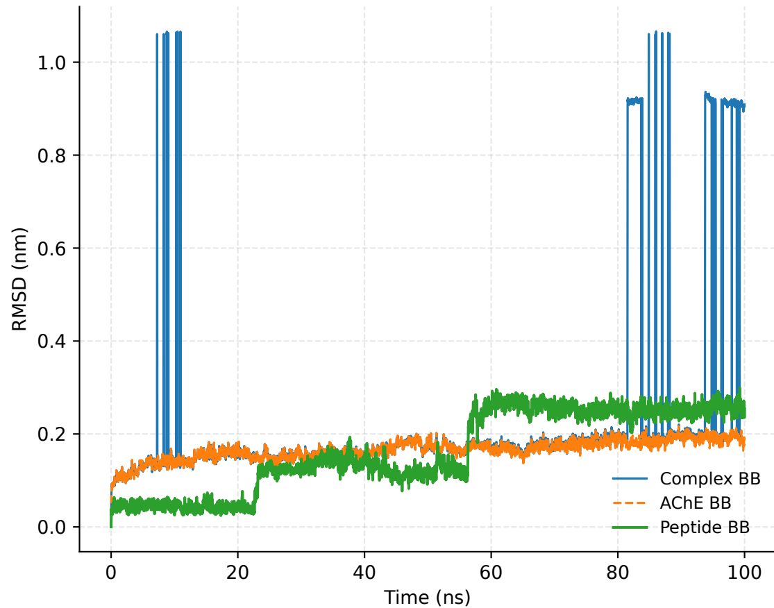
Backbone C \alpha RMSD
