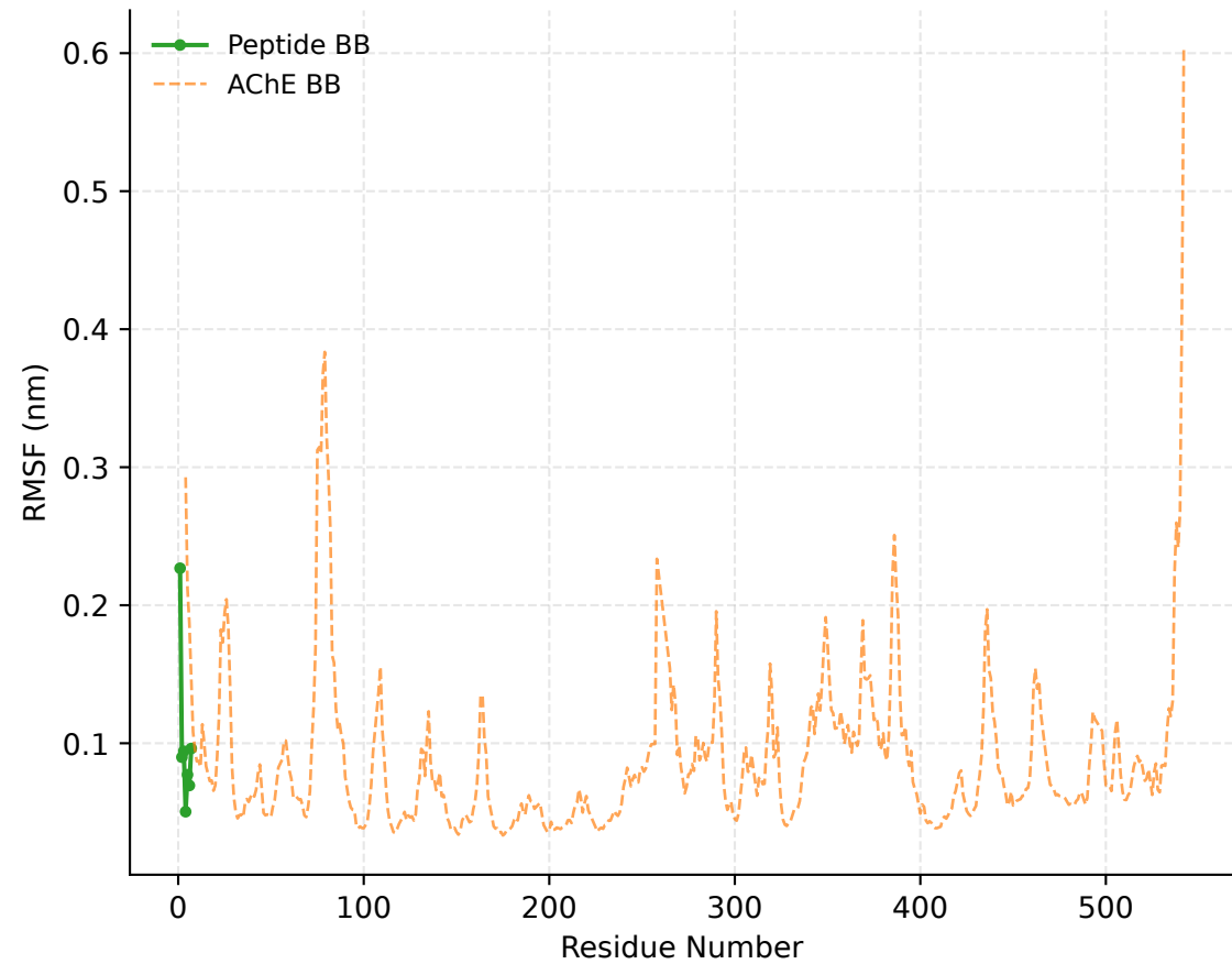
Backbone C \alpha RMSF
