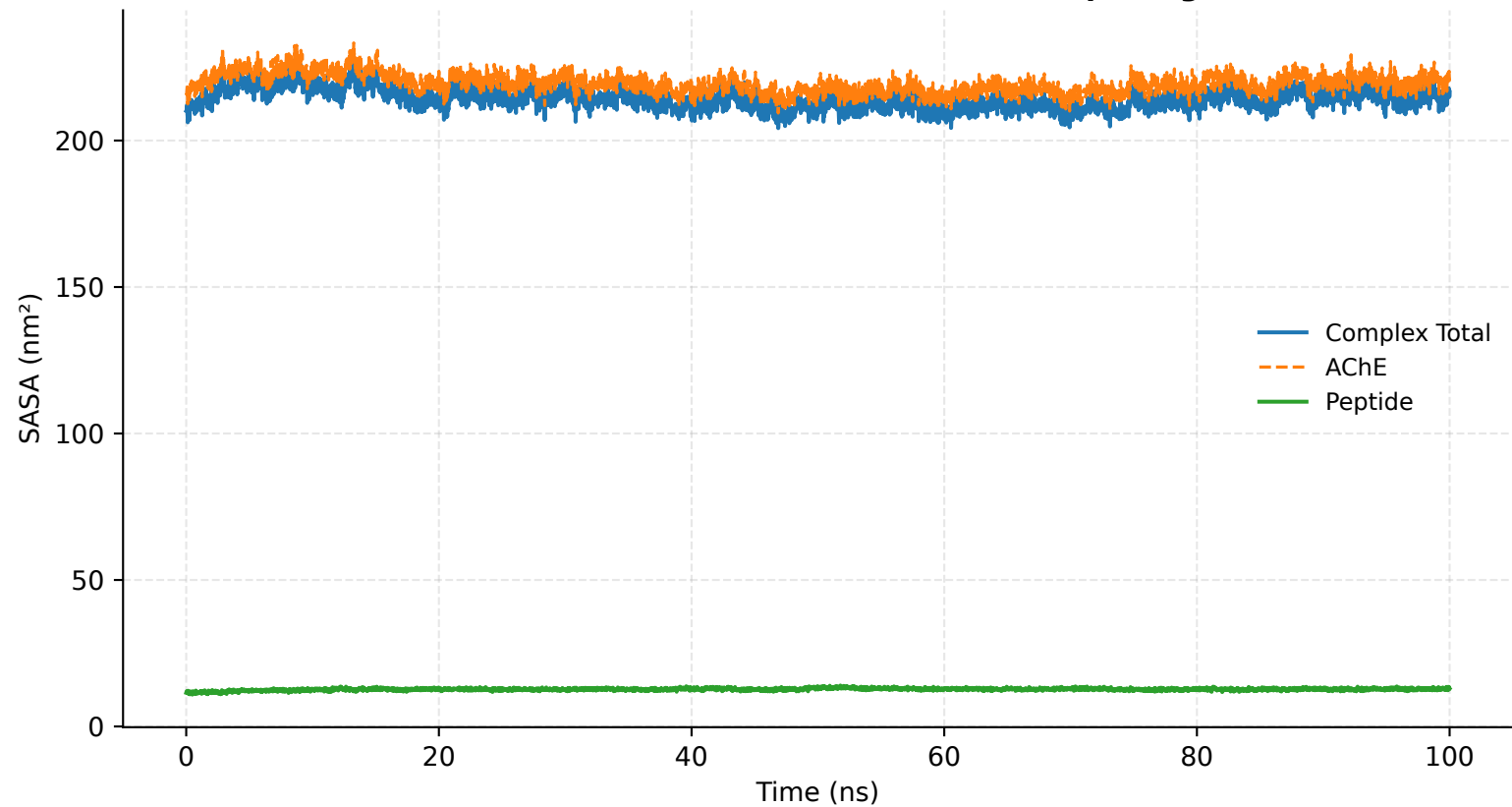
Solvent Accessible Surface Area (SASA, Paper Fig 3)
