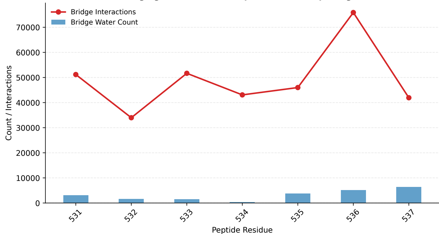
Bridging Water Molecules per Residue (Paper Fig 6)
