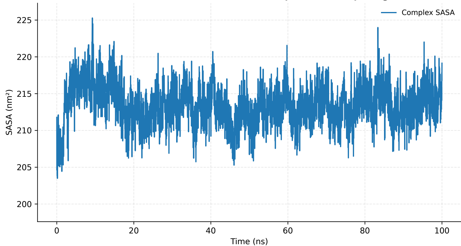
Solvent Accessible Surface Area (Complex SASA, Paper Fig 3)
