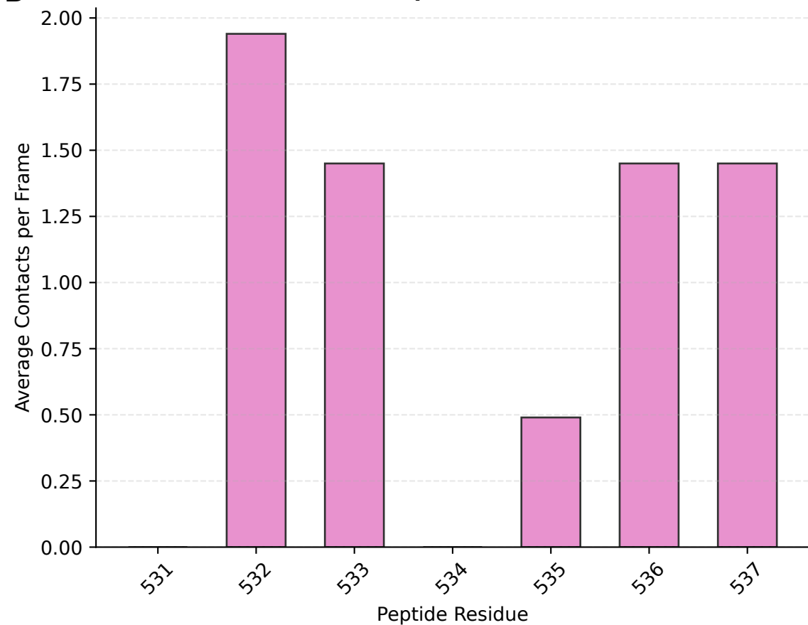
Intra-Peptide Contacts
