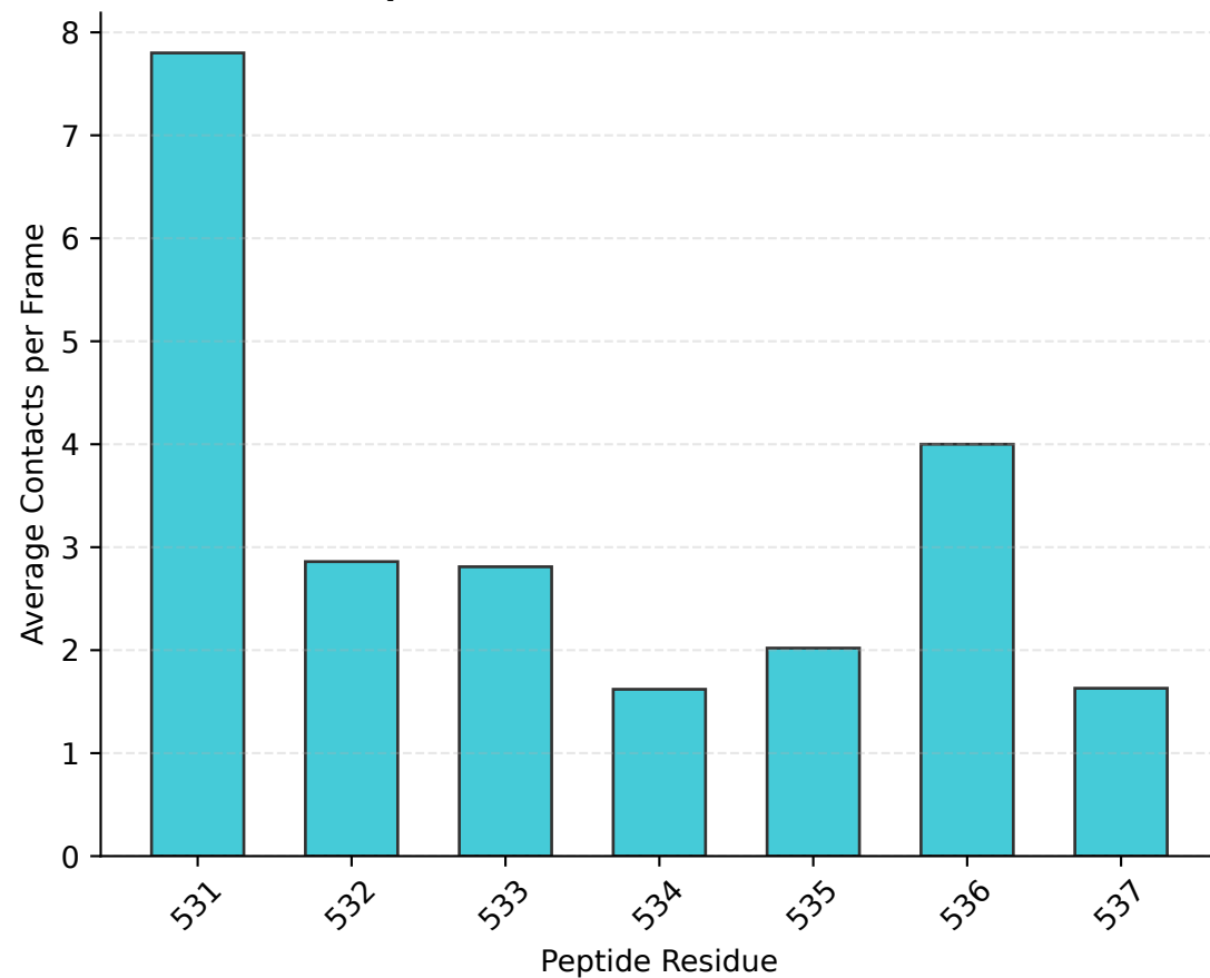
Peptide-AChE Non-Native Contacts
