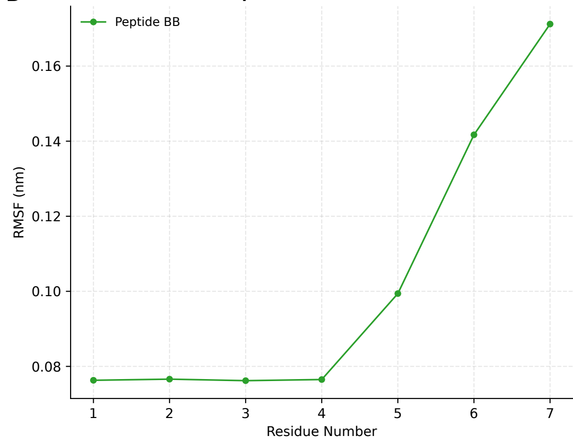
Peptide Backbone RMSF
