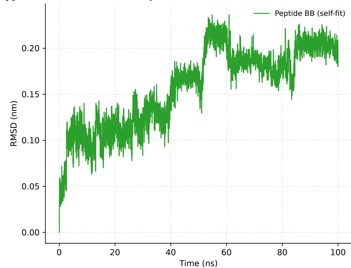
Peptide Backbone RMSD
