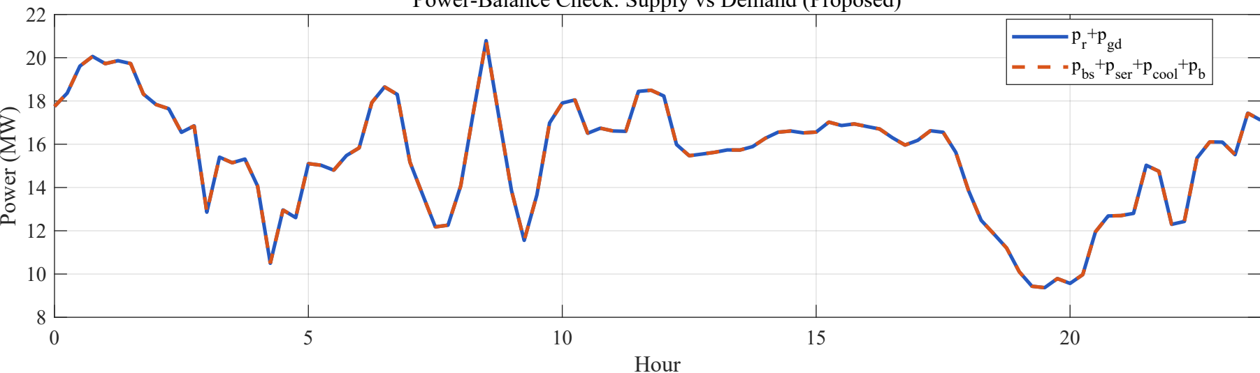
Power-Balance Check: Supply vs Demand (Proposed)
