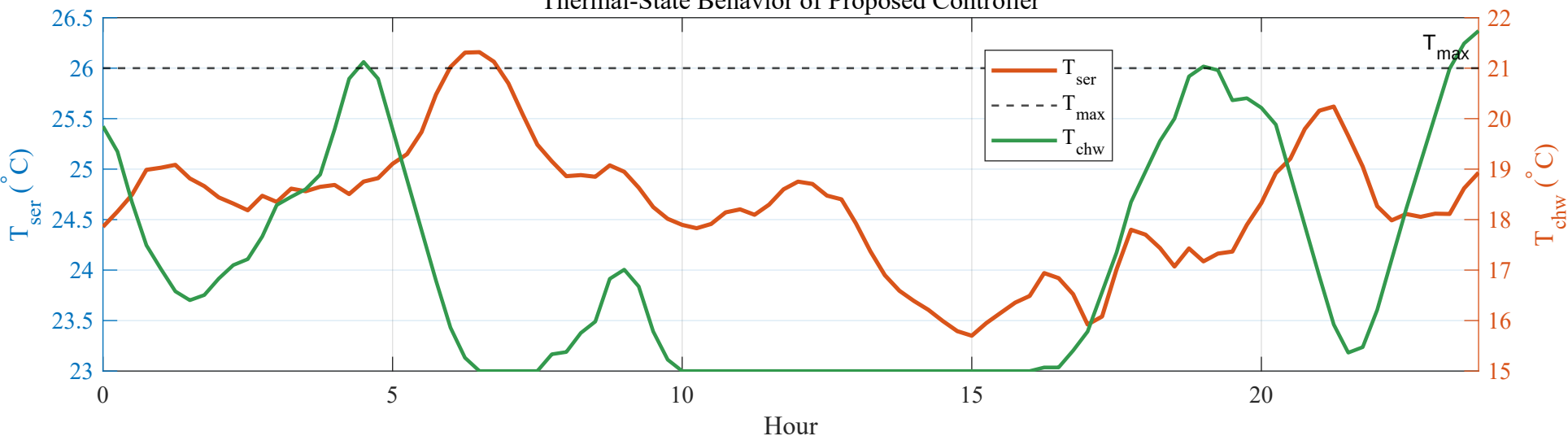
Thermal-State Behavior of Proposed Controller
