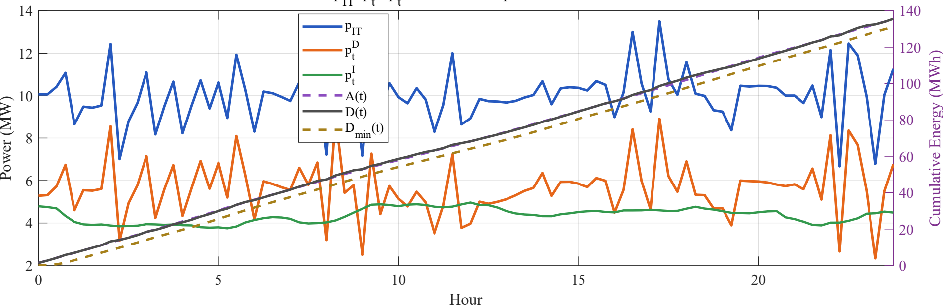
p_{IT} , p_t^D , p_t^I and Arrival-Departure Curves
