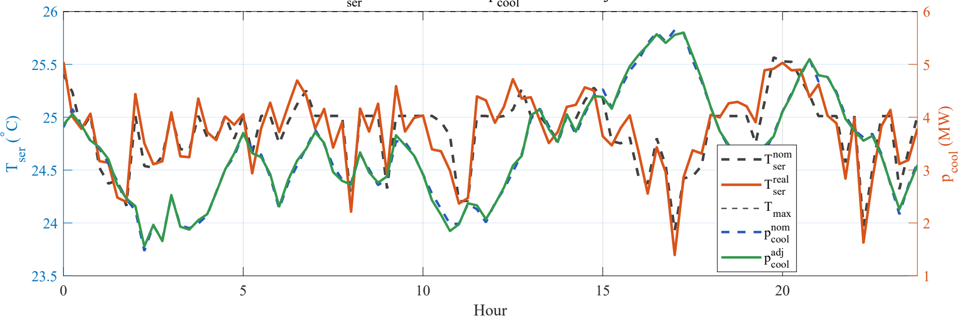
T_{ser} Nominal/Real and p_{cool} Nominal/Adjusted
