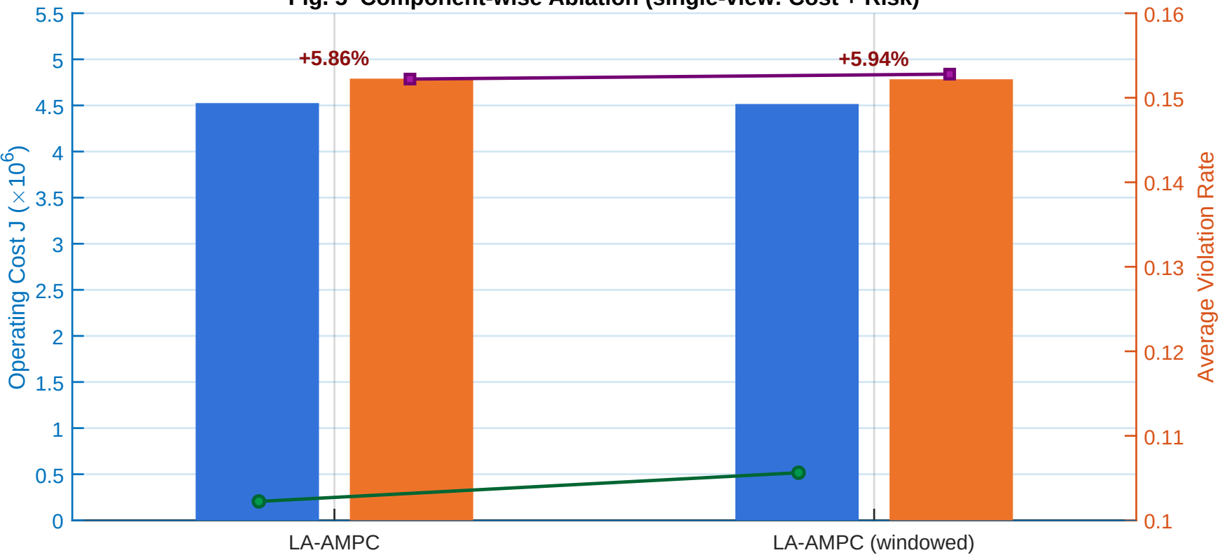
Fig. 5 Component-wise Ablation (single-view: Cost + Risk)
