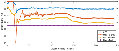
(b) CRAC unit setting temperature
