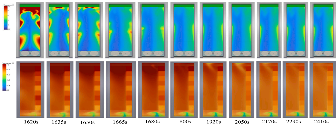
Fig. 10. Snapshots of servers temperature distribution when recover from abnormal.
