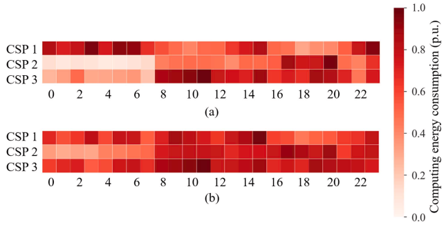
Fig. 10. The daily computing energy consumption of (a) heterogeneity-aware and (b) heterogeneity-agnostic CSPs.
