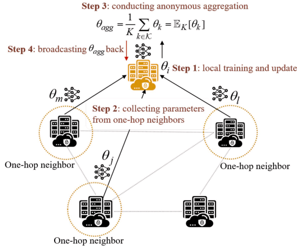
Fig. 3. Privacy-preserving training approach via FRL under the DTDE framework.
