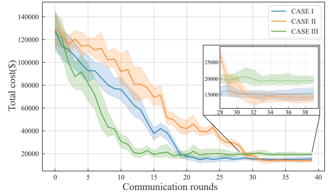
Fig. 8. Comparison of the training results in three cases.
