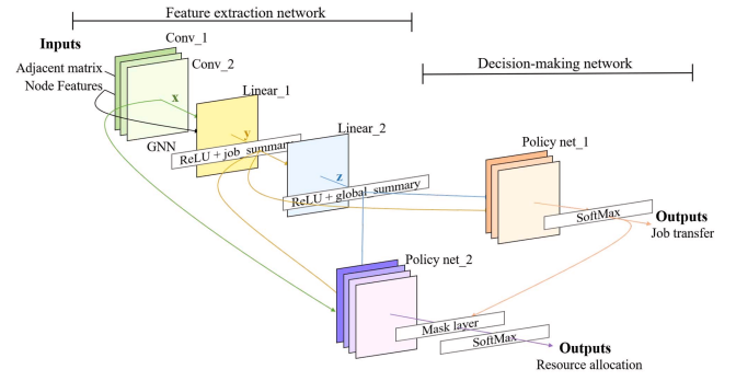
Fig. 2. CSP policy network architecture.
