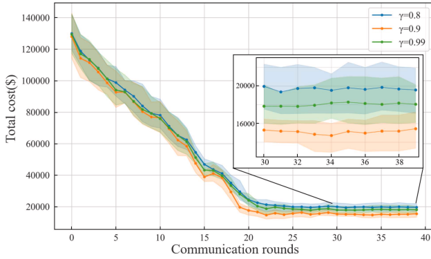
Fig. 11. Impact of the discount factor on the proposed method.
