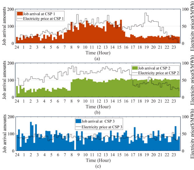
Fig. 4. Job arrivals and electricity prices at (a) CSP 1, (b) CSP 2, and (c) CSP 3.
