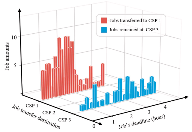
Fig. 6. A snapshot of CSP 3's job transfer decisions at 2:00.
