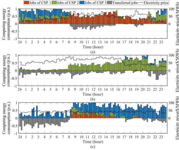
Fig. 5. Variations in the computing energy consumption of (a) CSP 1, (b) CSP 2, and (c) CSP 3.
