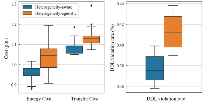
Fig. 9. Comparison of optimization results with and without heterogeneity-aware Scheduling.
