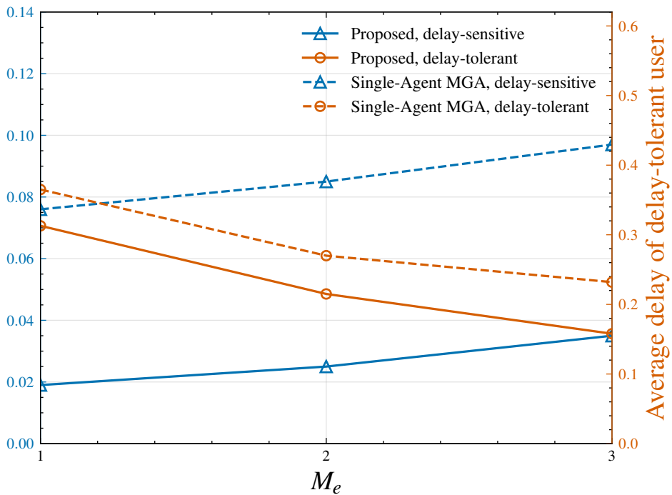
Outage ratio of delay-sensitive user
