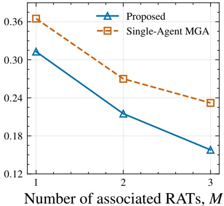
Average delay of eMBB
