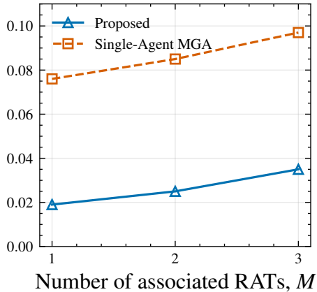
Outage ratio of URLLC
