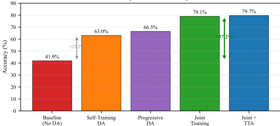
Domain Adaptation Method Comparison
