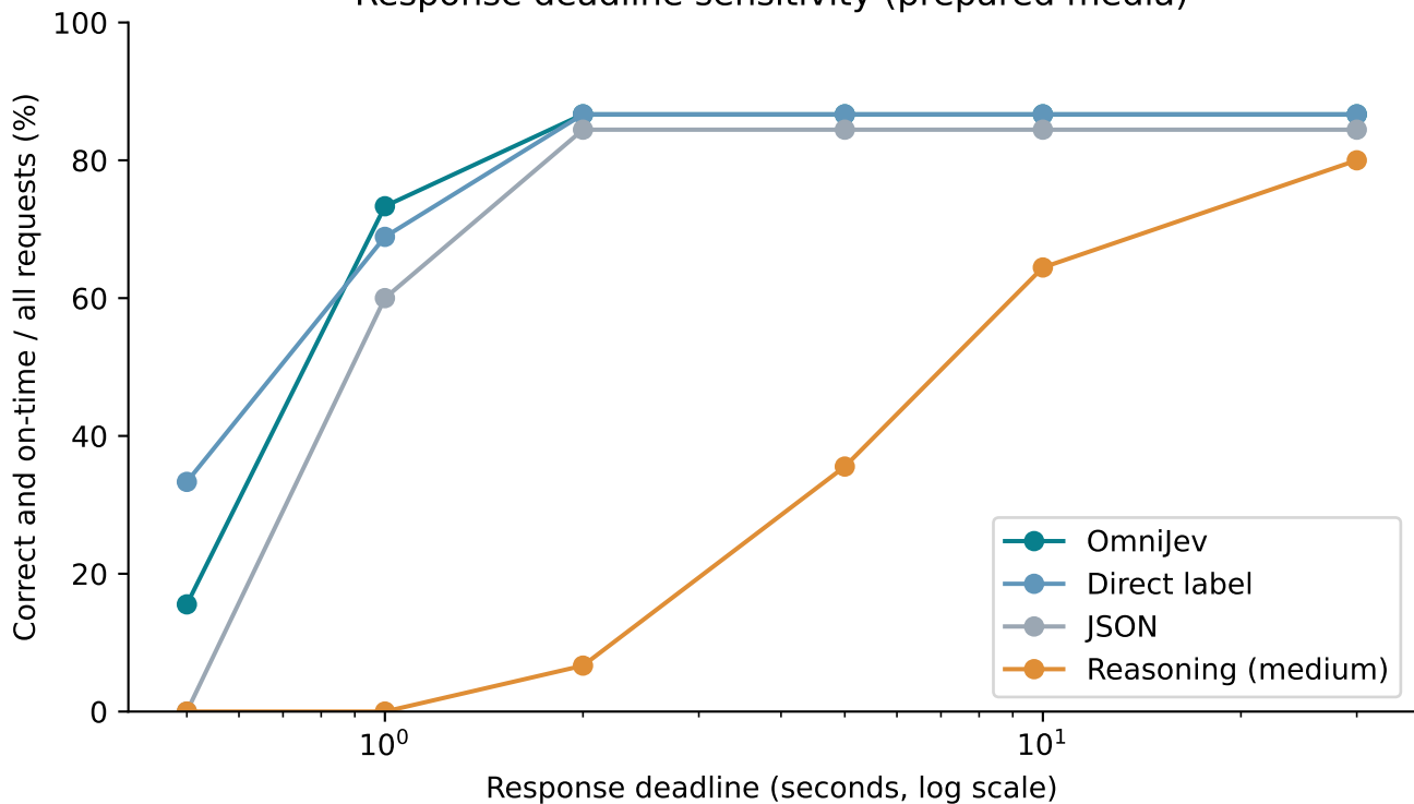
MMAD DS-MVTec zero-shot pilot | 45 cases Response deadline sensitivity (prepared media)
