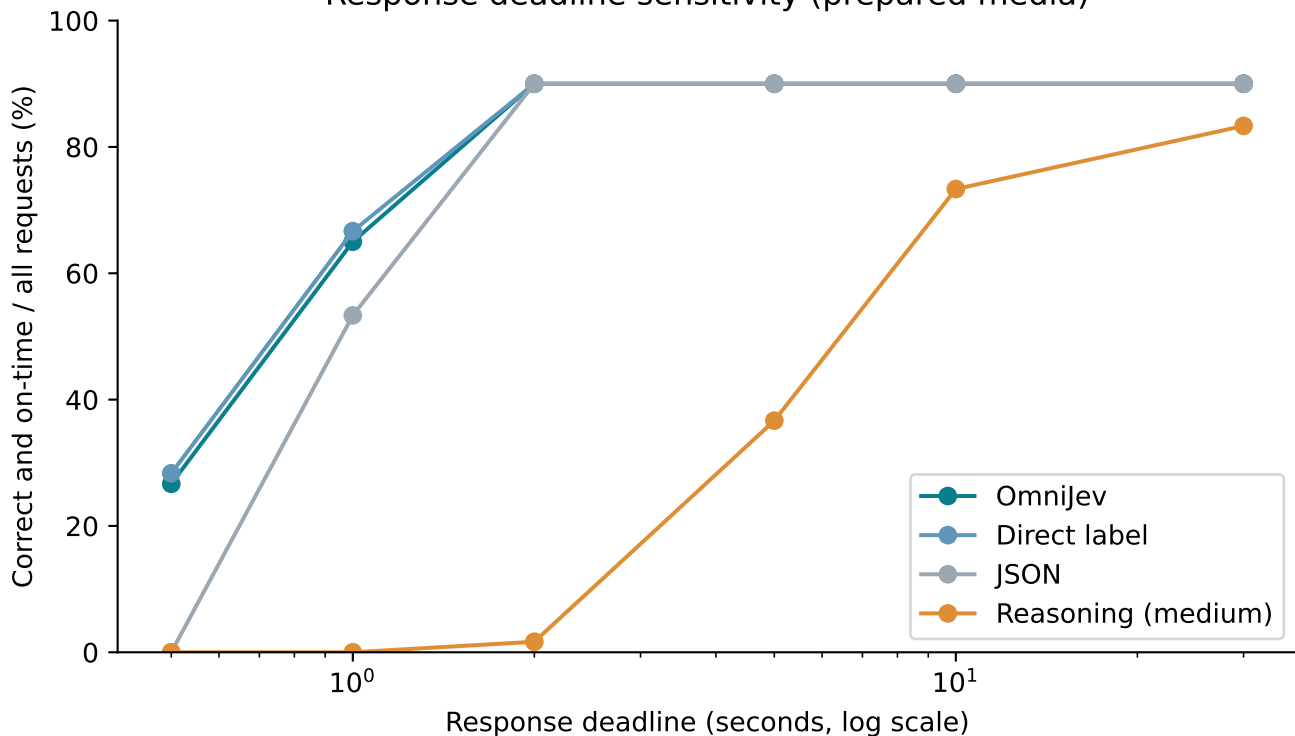
MMBench DEV EN pilot | 60 cases Response deadline sensitivity (prepared media)
