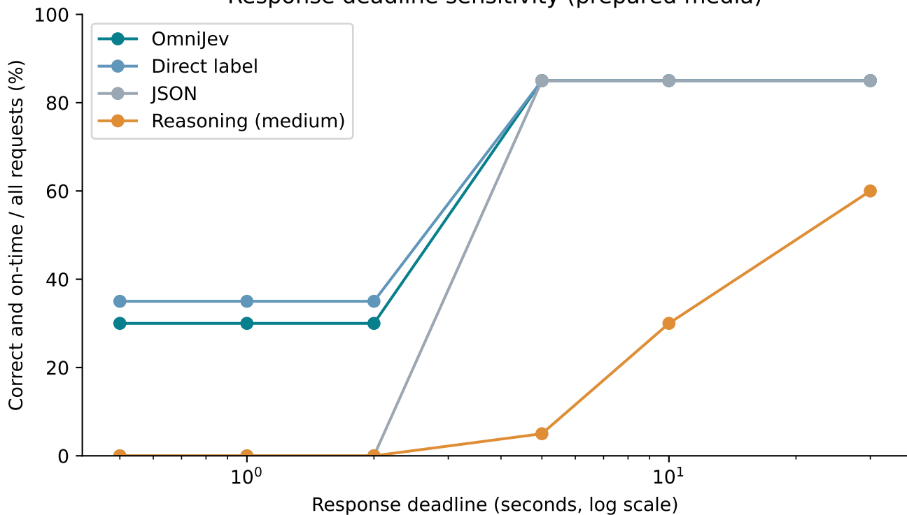
StreamingBench causal 8-frame pilot | 20 cases Response deadline sensitivity (prepared media)
