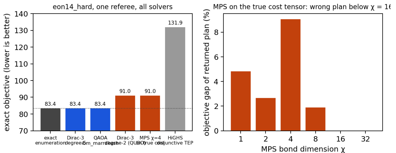
Figure 2 — Left: eon14_hard graded by the one referee for every solver — the device holding the full degree-5 polynomial and QAQA return the certified plan; the QUBO restriction and a \chi=4 MPS return the same wrong plan. Right: MPS on the true cost tensor returns the wrong plan at every \chi below 16.
